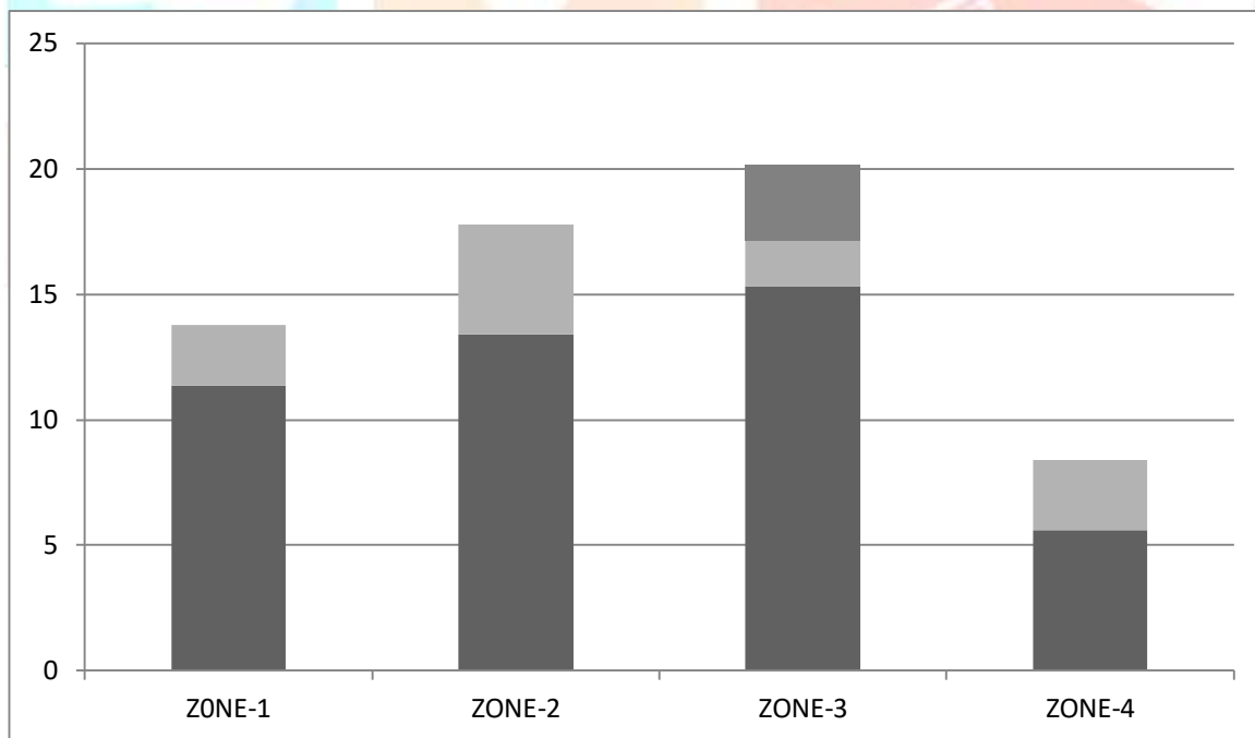
ONE WAY ANOVA CALCULATOR (ONLINE MODE)
