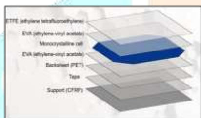
Fig 1. Different layers of solar panel
