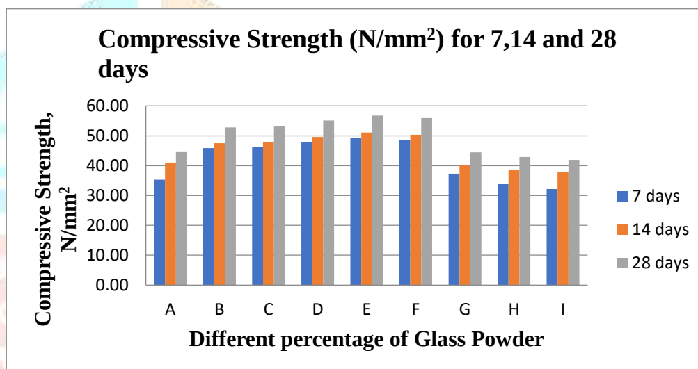
Chart - 1: Compressive strength of cube (N/mm 2 ) for 7 days, 14 days and 28 days
