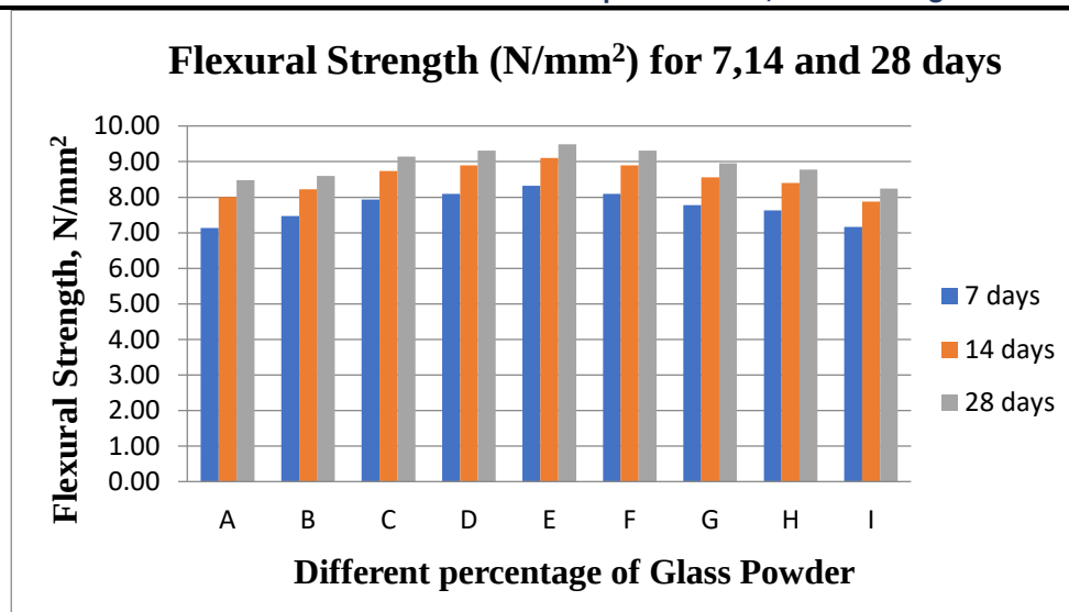
Chart - 2: Flexural strength of cube (N/mm 2 ) for 7 days, 14 days and 28 days
