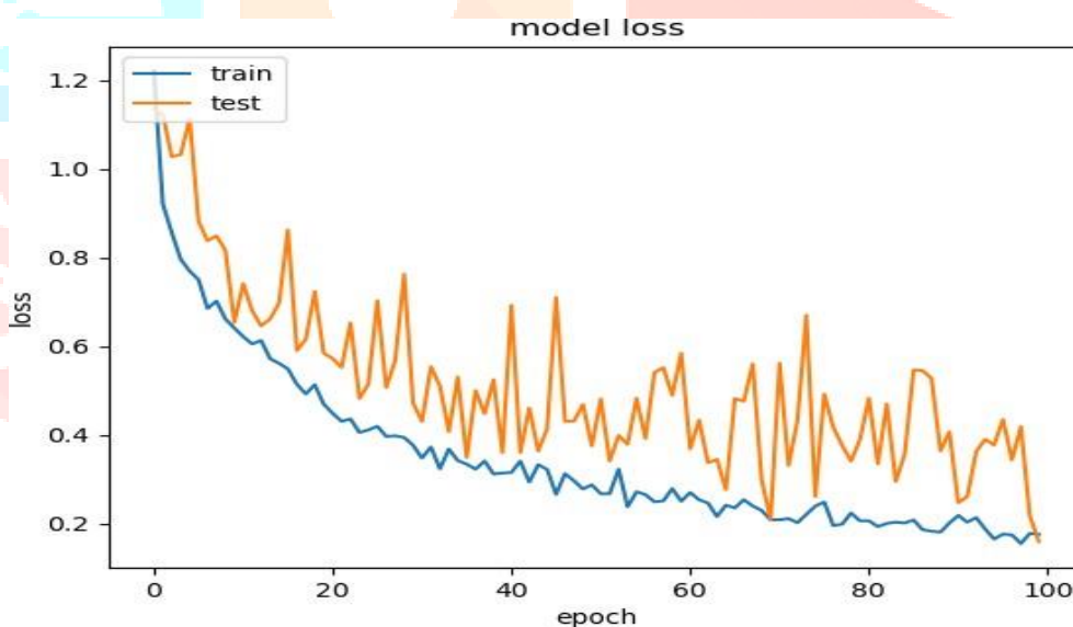
Fig. 4. Model loss
