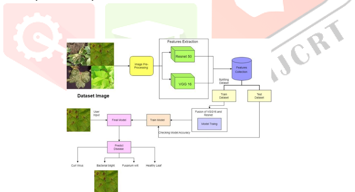
Fig. 1. Block diagram [ Using Algo VGG16 and Resnet50]
