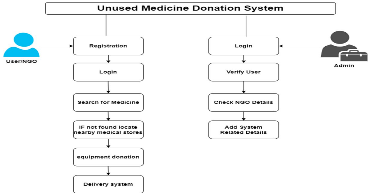
Diagram 4.1.System Architecture
