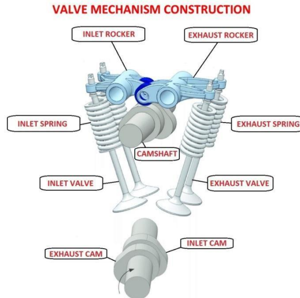
Figure 1.2. Valve mechanism
