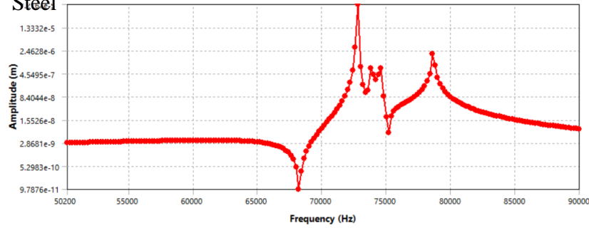
Figure 4.2. Frequency response curve of closing cam for stainless steel
