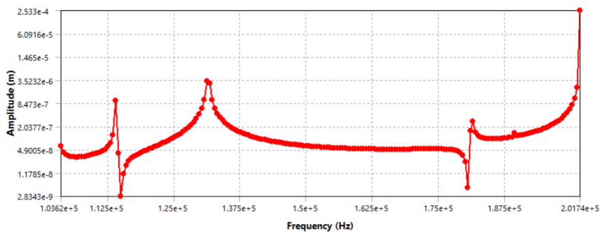
Figure 4.4. Frequency response curve of opening cam for Structural Steel
