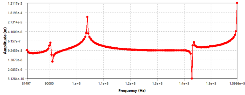
Figure 4.1. Frequency response curve of opening cam for Stainless Steel
