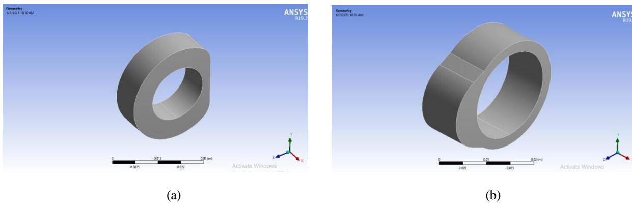
Figure 3.2.1. (a) Geometry of closing cam, (b) Geometry of opening cam
