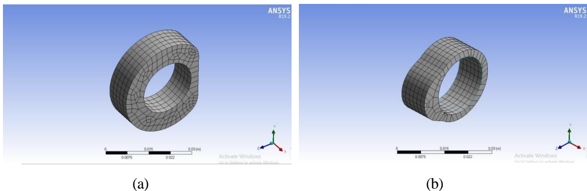
Figure 4.2.2. (a) Represent meshing of closing cam, (b) Represent meshing of opening cam
