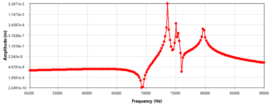
Figure 4.6.. Frequency response curve of closing cam for structural steel
