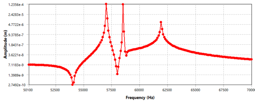
Figure 4.3 Frequency response curve of closing cam for Gray Cast Iron
