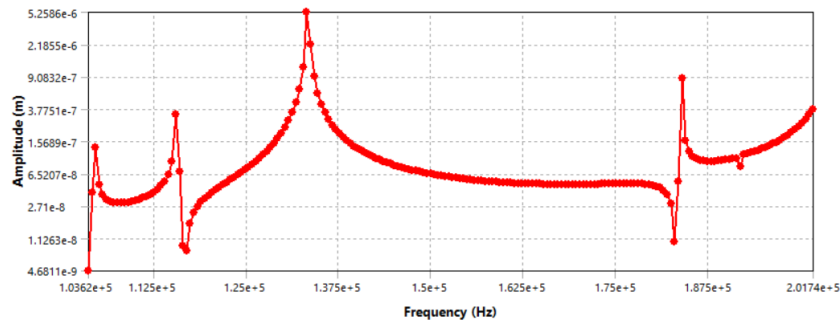
Figure 4.5 Frequency response curve of opening cam for Gray Cast Iron
