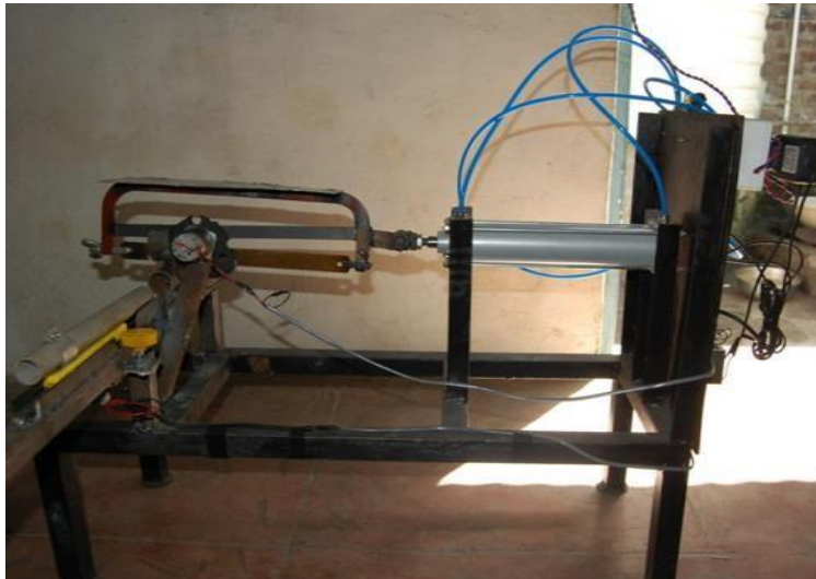
Figure 1 Pneumatic cutting machine
