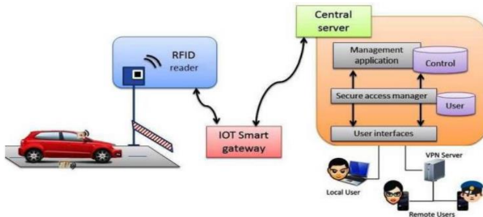
Fig 1. IOT BASED SMART PARKING SYSTEM
