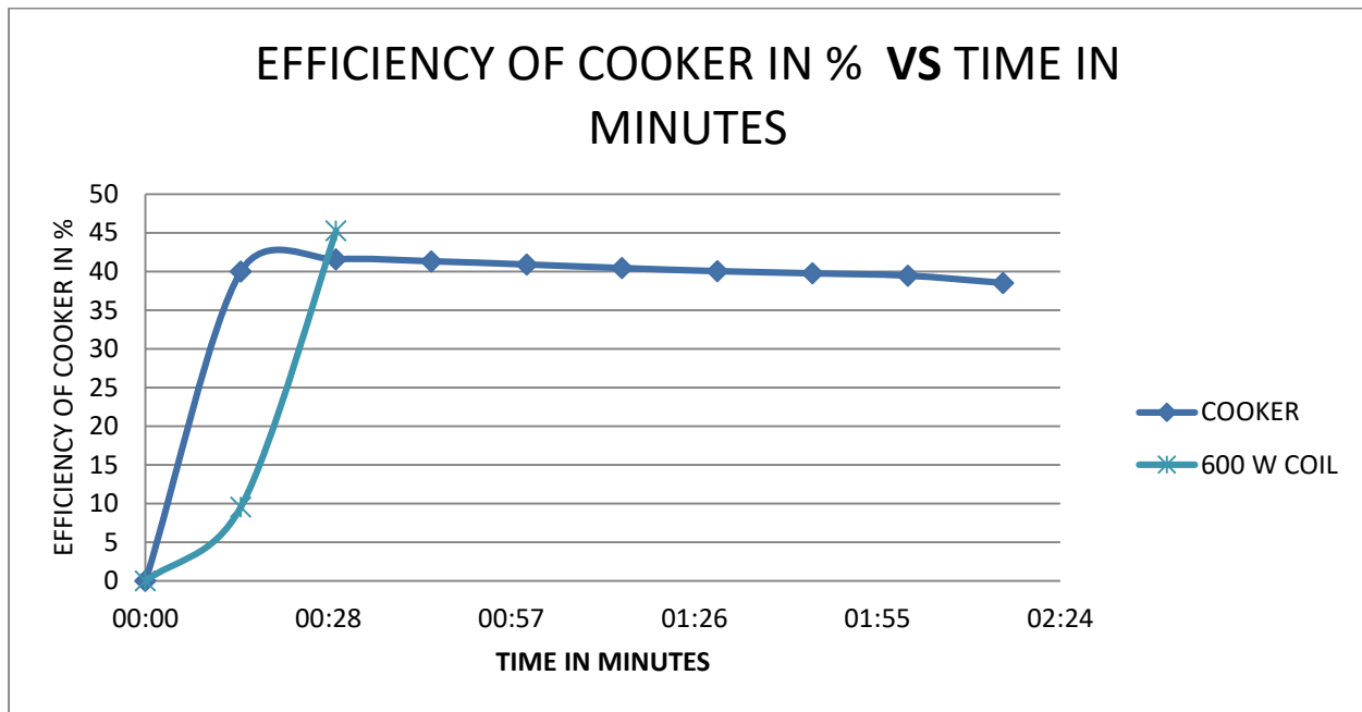
Fig.3. Variation efficiency of solar cooker and time taken to efficiency of solar cooker
