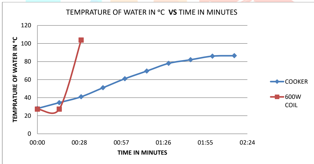
Fig.2. Variation of water temperature and time taken to reach the water temperature
