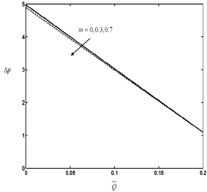
Fig. 13(i) The variation of the pressure rise \Delta p with \bar{Q} for different values of m with n=0.5, \beta=0.1, We=0.01, Da=0.1, M=1 and \phi=0.6 .
