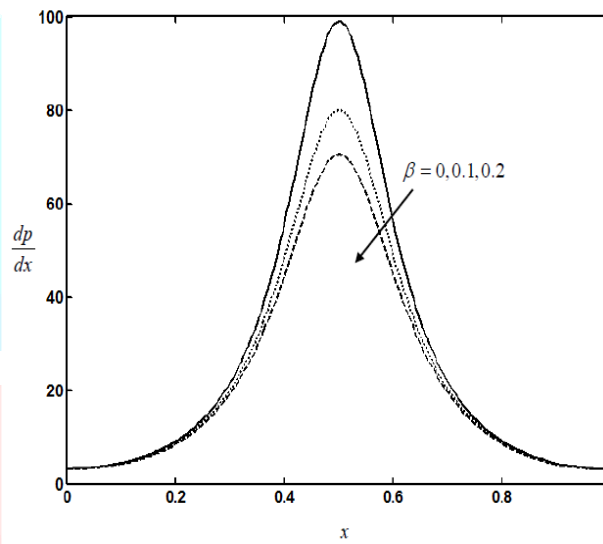
Fig. 4 The variation of the axial pressure gradient \frac{dp}{dx} with \beta for n=0.5, We=0.01, M=1, m=0.2, Da=0.1, \phi=0.6 and \bar{Q}=-1 .
