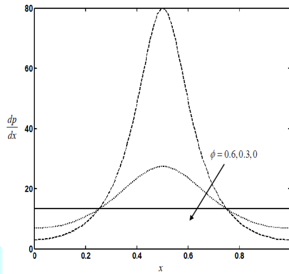
Fig. 8 The variation of the axial pressure gradient \frac{dp}{dx} with \phi for n=0.5, m=0.2, M=1, \beta=0.1, Da=0.1, We=0.01 and \bar{Q}=-1 .
