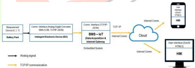
Fig. 6. Proposed Blockdiagram of a IoT Battery pack
