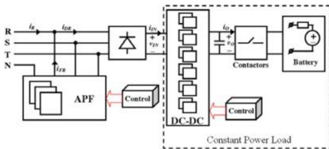
Fig. 3. Block Diagram for DC fast charging implementation
