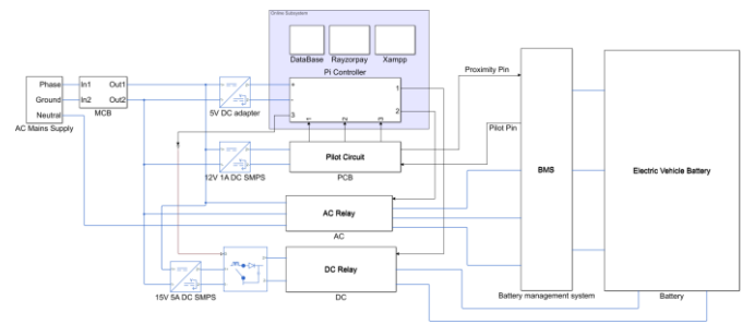
Fig. 9. Functional Block Diagram of system
