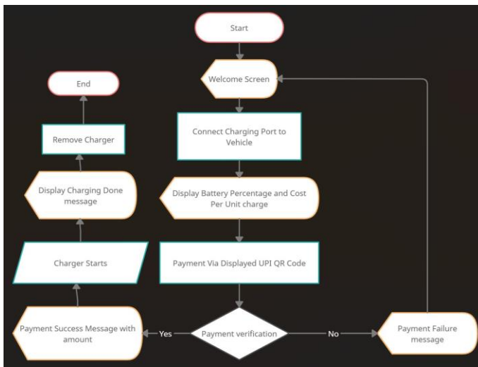
Fig. 8. Client Side Flow
