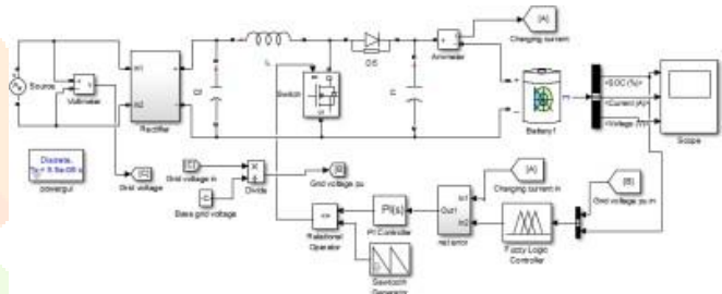
Fig. 4. Simulation for Smart DC fast charging
