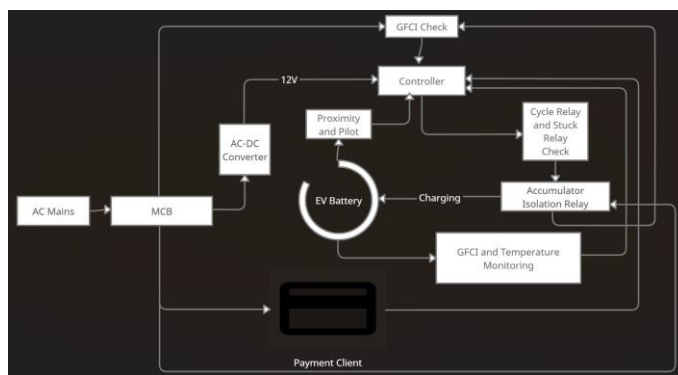
Fig. 12. Diagram showing the flow of data in the system
