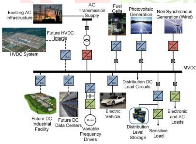
Fig. 5. Implementation of Medium Voltage DC Grid for a Network of Stations
