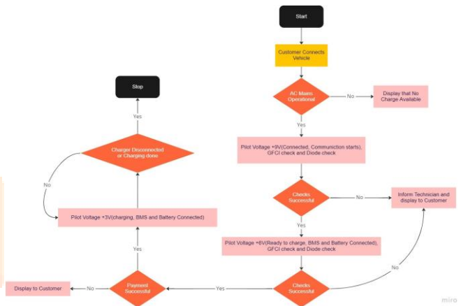
Fig. 16. Pilot Algorithm
