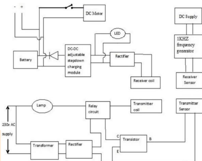
Fig. 1. Proposed Block Diagram of Smart Charging for Electric Vehicles
