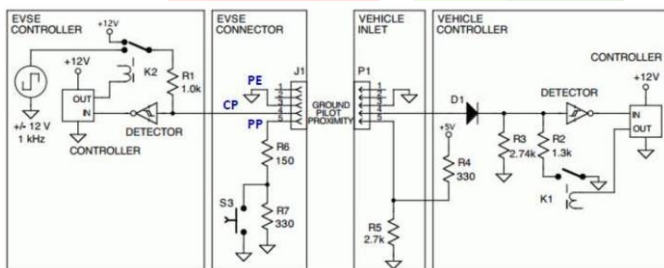
Fig. 22. J1772 Standard EV Charging Connections
