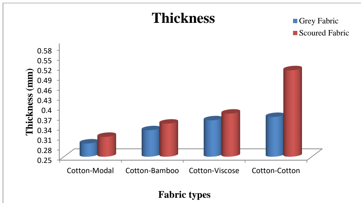
Fig.2 Thickness of grey and scoured fabrics
