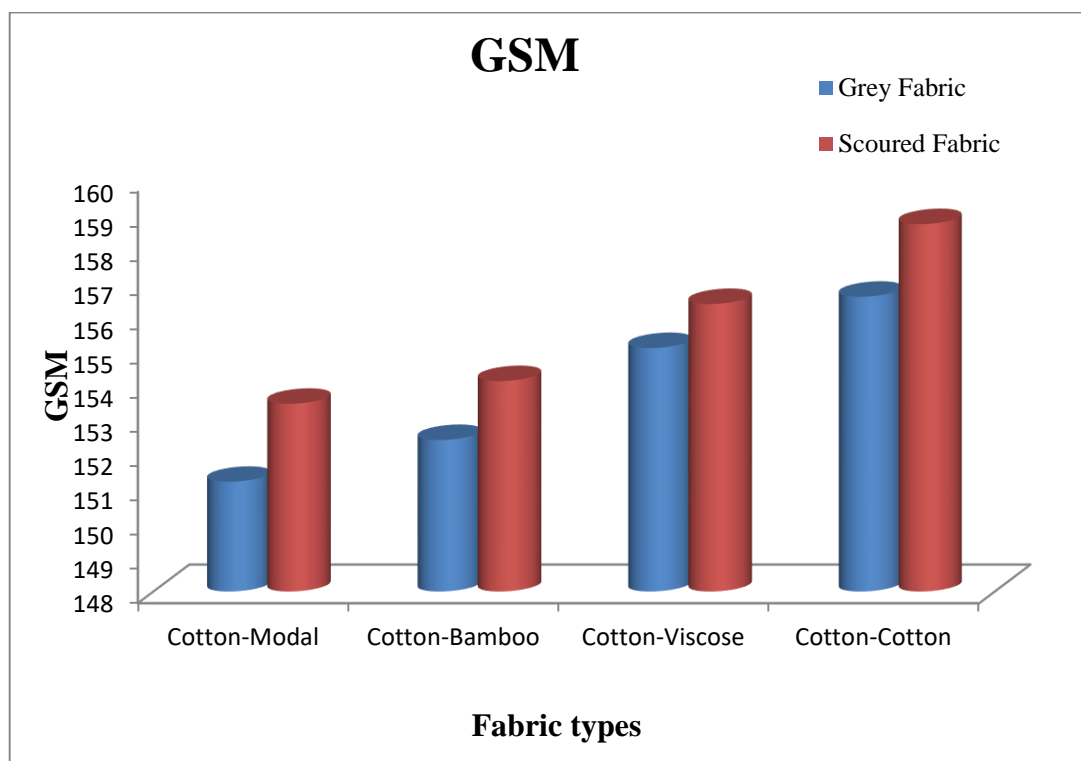
Fig 1 GSM of grey and scoured fabrics
