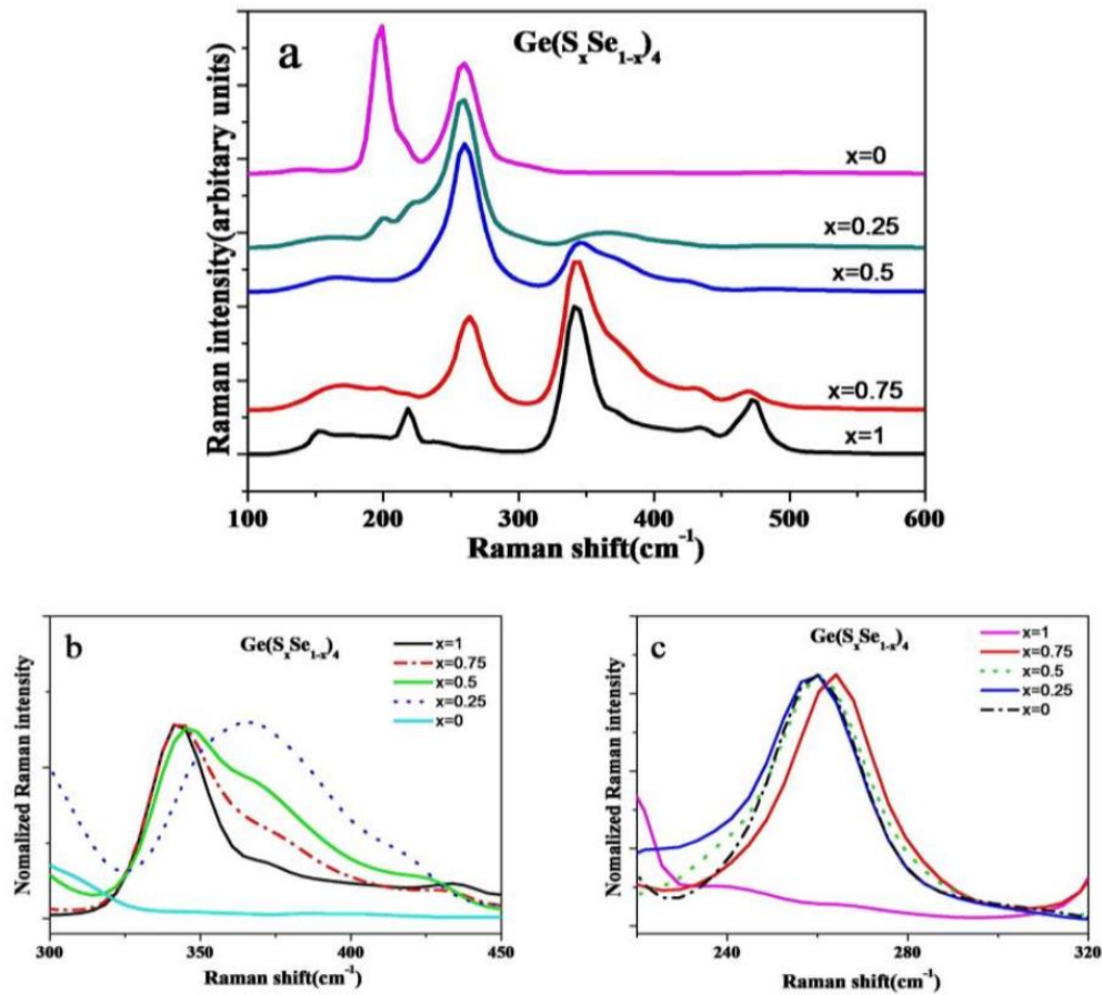
Fig.1 The experimental Raman spectra of the \text{Ge}(\text{S}_x\text{Se}_{1-x})_4 glassy system, x=0, 0.25, 0.5, 0.75, 1 , b is obtained by normalization processing of peaks positing near 340 \text{ cm}^{-1} , c is obtained by normalization processing of peaks positing near 260 \text{ cm}^{-1}
