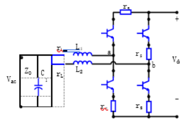
Figure8.TheequivalentcircuitinDC/ACmode
