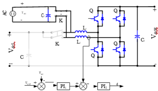
Figure 9: DC/ACmode.
