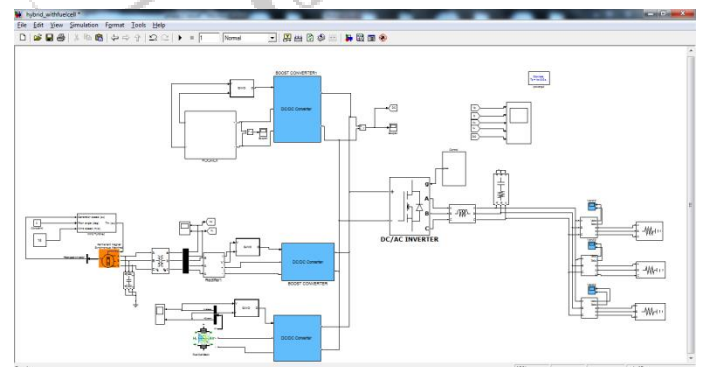
FIGURE. 2PROPOSED PCMM TOPOLOGY
