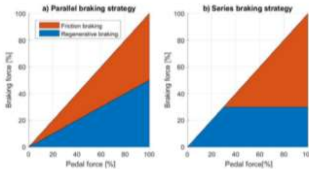
Fig 2. Division of braking forces into frictional braking and regenerative braking: a) Parallel strategy; b) Serial strategy
