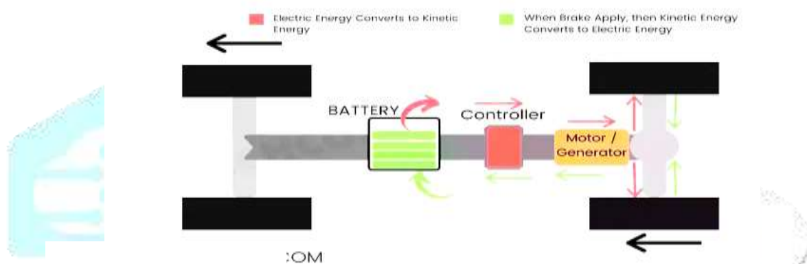
Figure 1 Block Diagram of Regenerative Braking System
