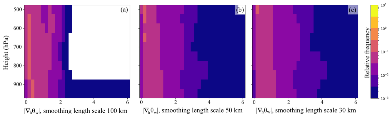
Figure 4. Distribution (relative frequencies) of |\nabla^* \theta_w| within frontal zones between 950-500 hPa (same data, time, and region as in Figure 3) for different smoothing length scales: (a) 100 km, (b) 50 km, and (c) 30 km.
