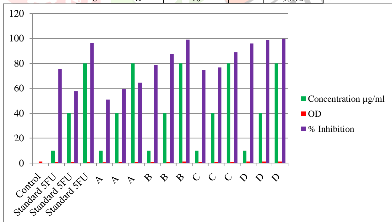
Fig.3: At the Concentration 80µg/ml, sample Code A, B, C, D samples showed good percent inhibition MCF7cell line as compared to standard drug.
