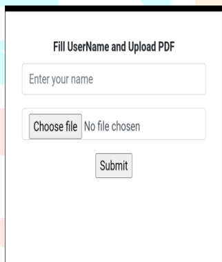
Fig 1.3 upload document
