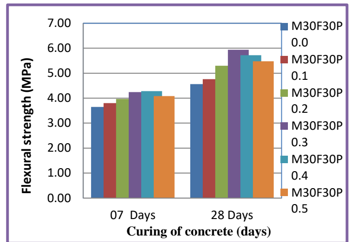
Figure 5: Variation of Flexural Strength with age for M30 grades with varying proportions WPF for 60mm thick paver block
