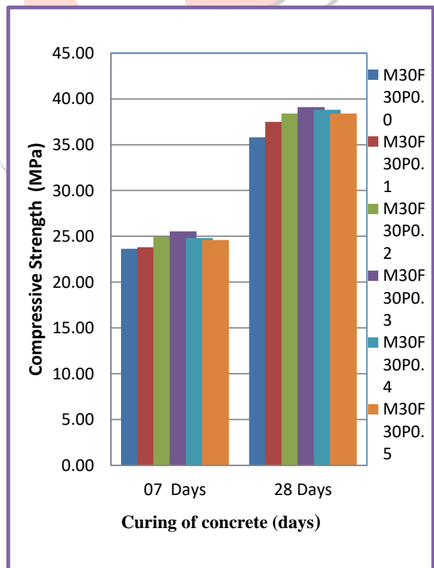
Figure 4: Variation of corrected compressive strength with age for M30 grades with varying proportions WPF for 60mm thick paver block
