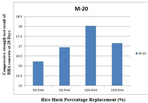
Graph-11: 28 days compressive strength of concrete for M-20 grade concrete Graph-12: 28 days compressive strength of concrete for M-25 grade concrete
