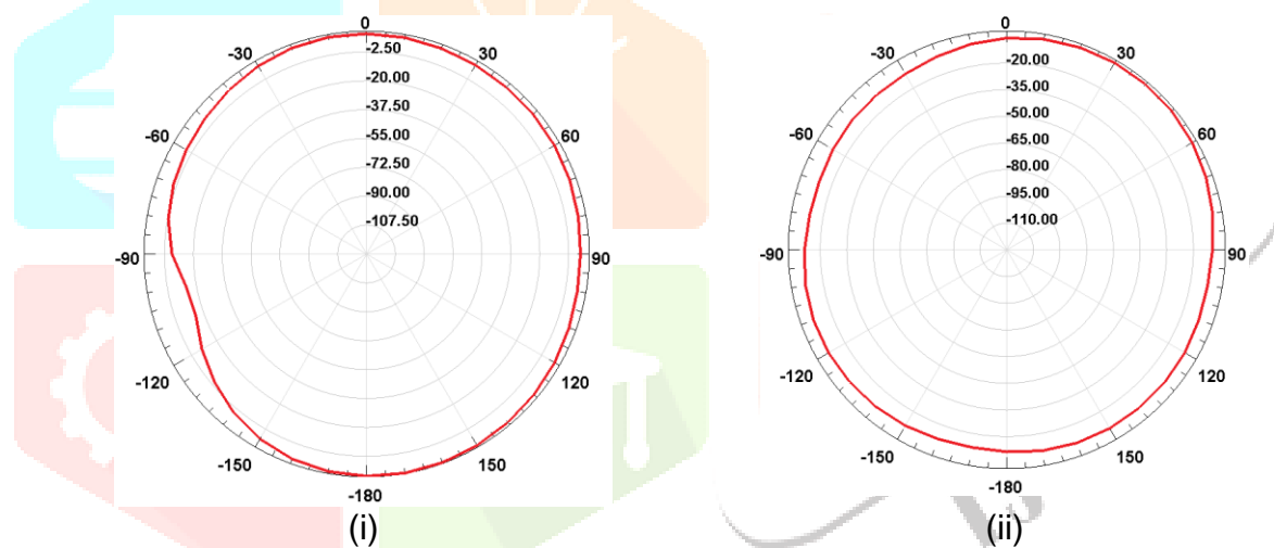
Figure 4: 2D radiation pattern at 3.10 GHz and 4.33 GHz frequencies.
