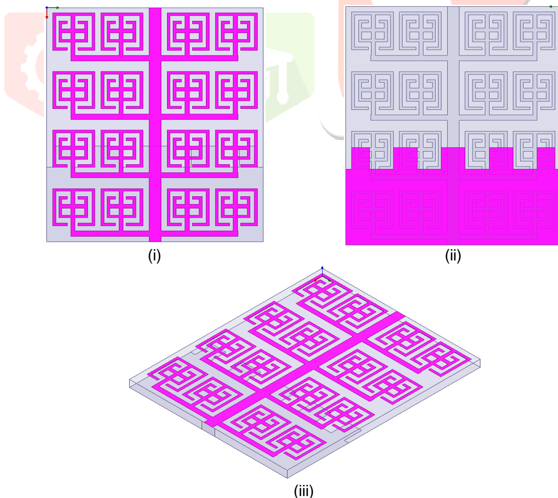
Figure 2: (i) Top View (ii) Back View (iii) Bird-eye View
