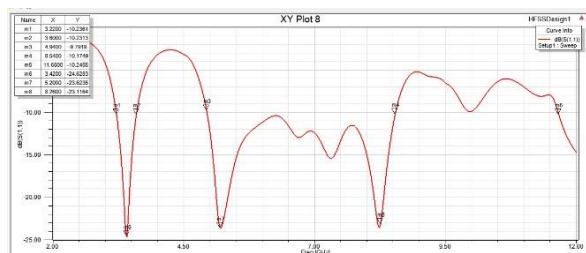
Figure 3 Simulated return loss curve of proposed antenna.
