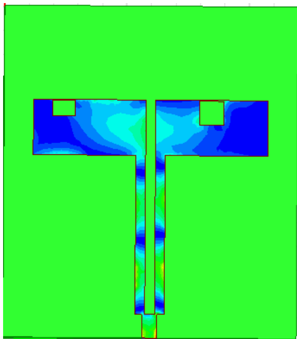
Figure 5 Surface current distribution of the proposed at (5.25)
