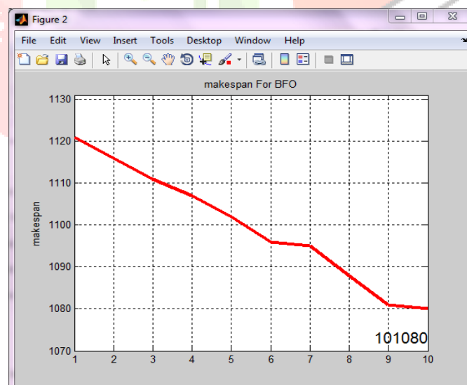
Figure 6.1 Makespan for 100 jobs and 70 virtual machines
