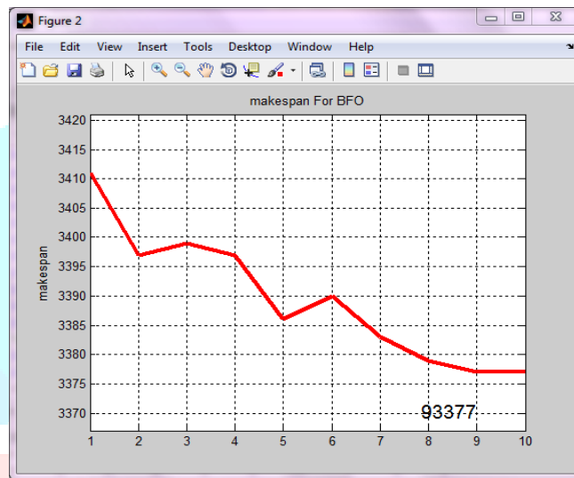
Figure 6.3 Makespan for 200 jobs and 70 virtual machines
