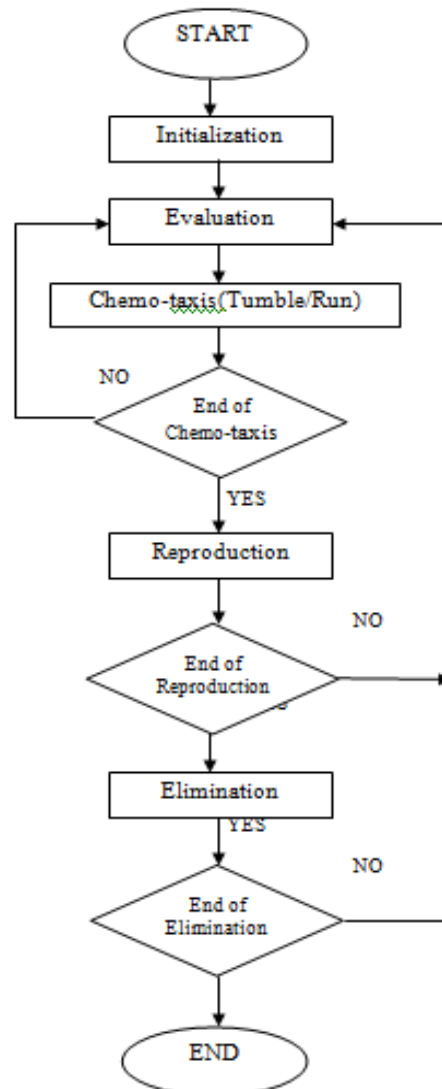
Figure 2.2: Flowchart of BFOA
