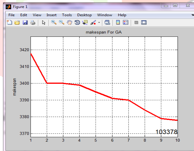
Figure 6.4 Makespan for 500 jobs and 70 virtual machines
