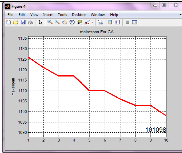
Figure 6.2 Makespan for 100 jobs and 70 virtual machines
