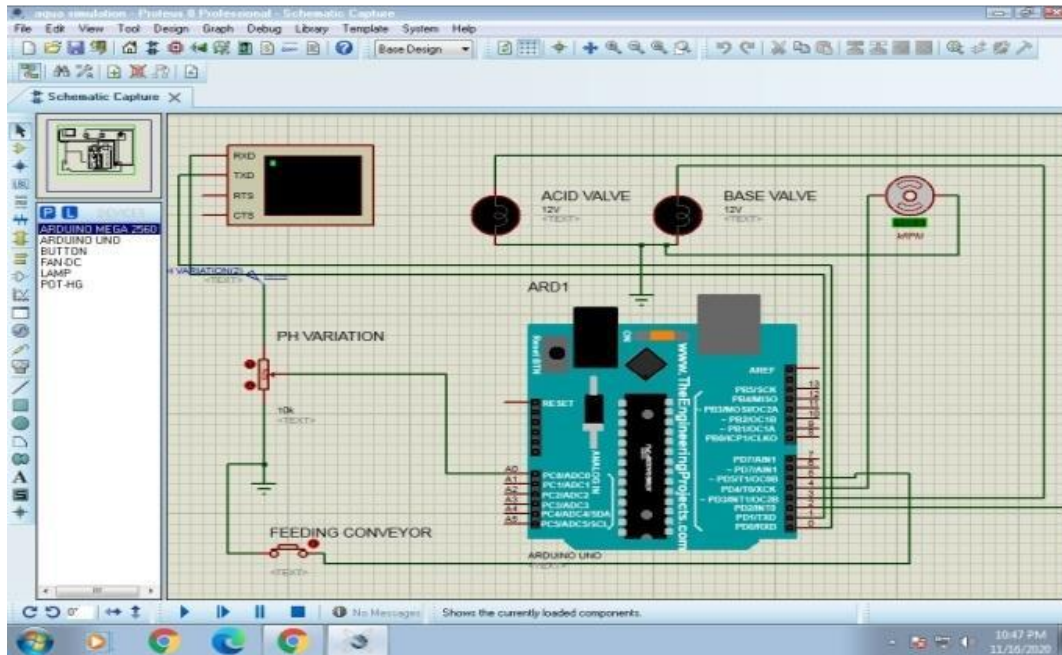
Fig.4. Simulation window
