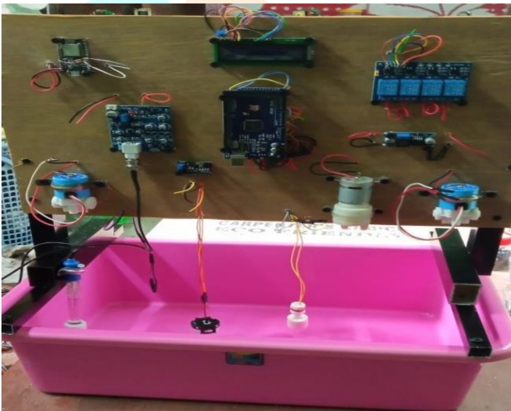
Fig.2.Hardware implementation
