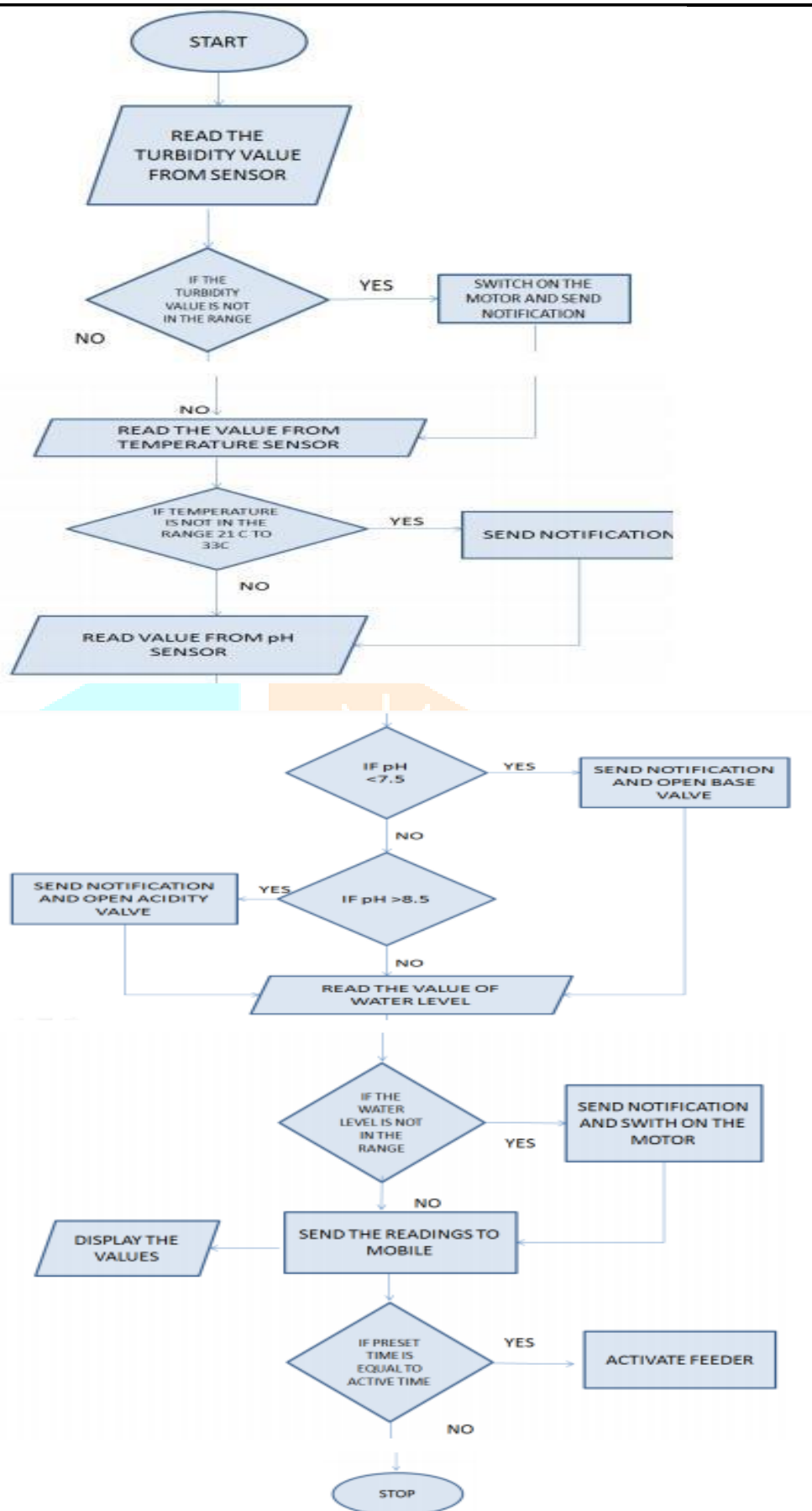
Fig.3. Flow chart for the proposed model
