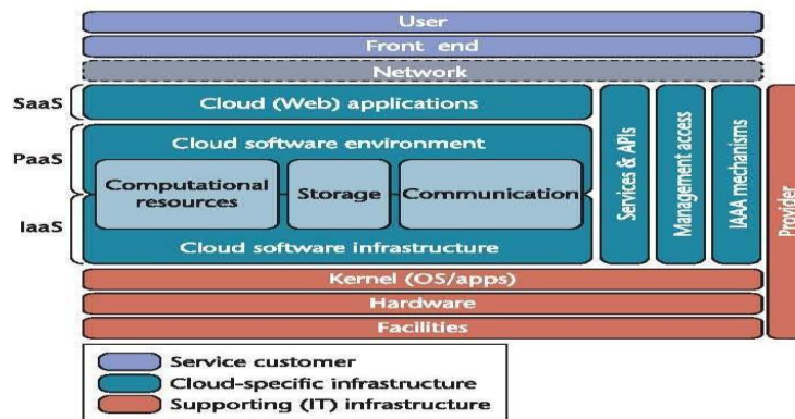
Fig.1 Cloud Reference Architecture
