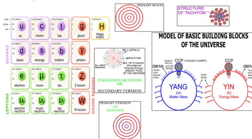
Standard model completed with Fundamental particles and Mind And Tachyons
