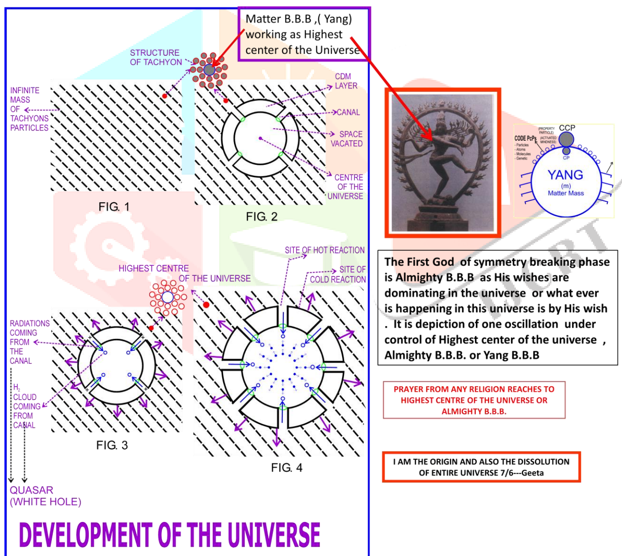
Figure 9.1 Hoyle Narlikar Universe OR Universe “I”
