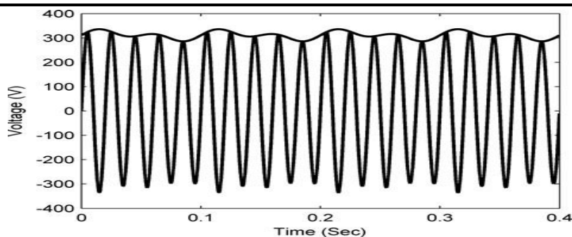
FIGURE 8:- VOLTAGE FLICKER
