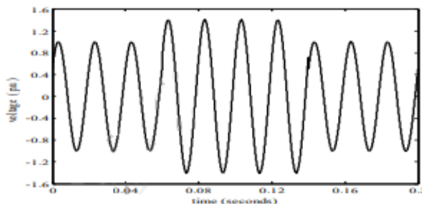
FIGURE 2:- VOLTAGE SWELL
