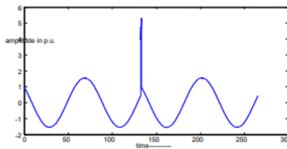
FIGURE 4:- IMPULSIVE TRANSIENT
