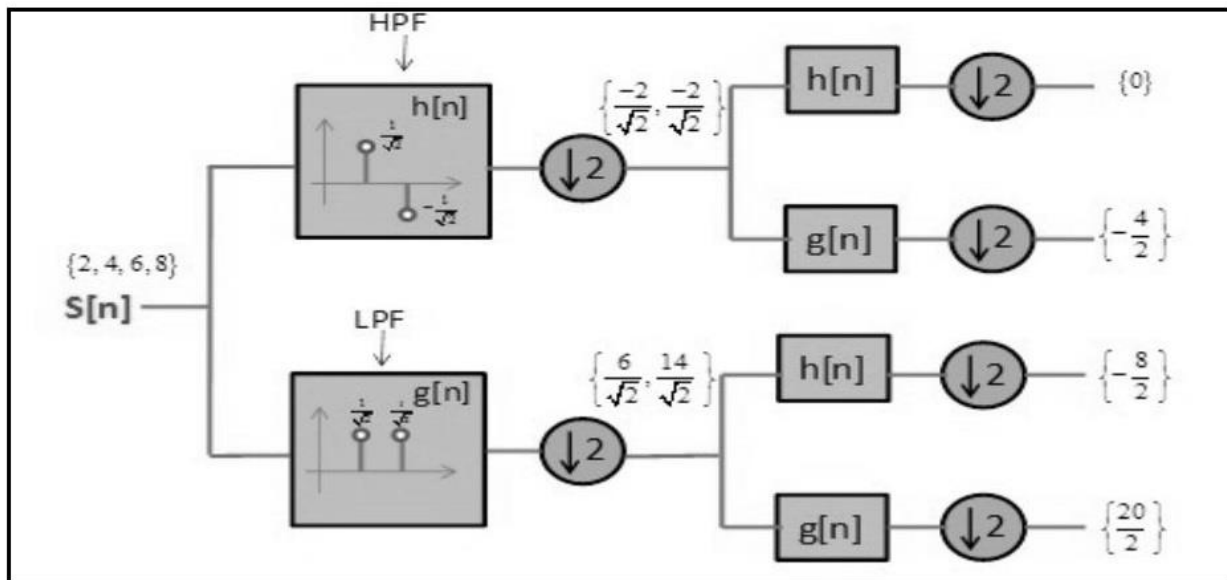
Figure 9:- Two level wavelet packet decomposition
