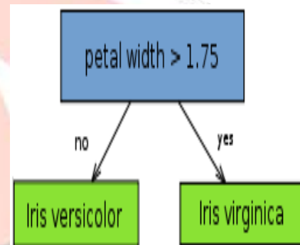
Figure 2: Decision Stump Model
