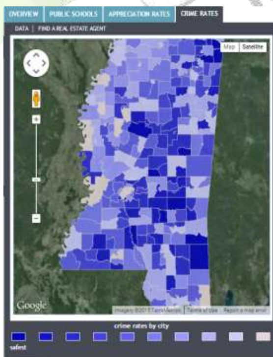
Figure 5: Crime Rates in Different Cities of Mississippi
