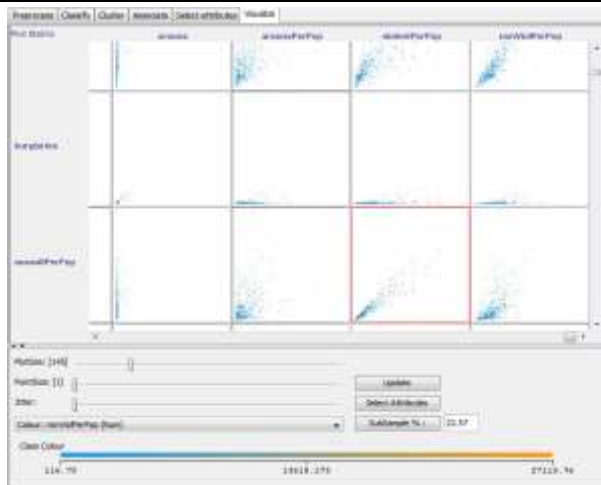
Figure 3: Plot Matrix
