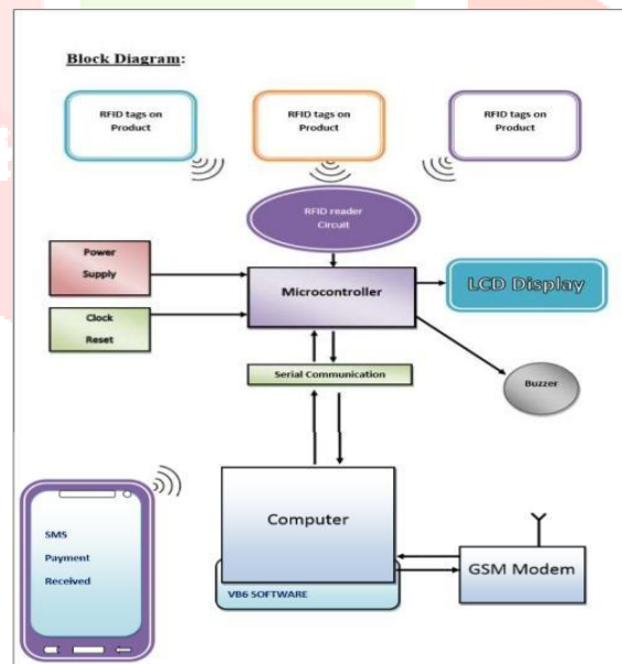
Fig.1 ProposedSystem
