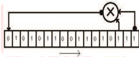
Figure 1: Linear Feedback Shift Register (LFSR).
