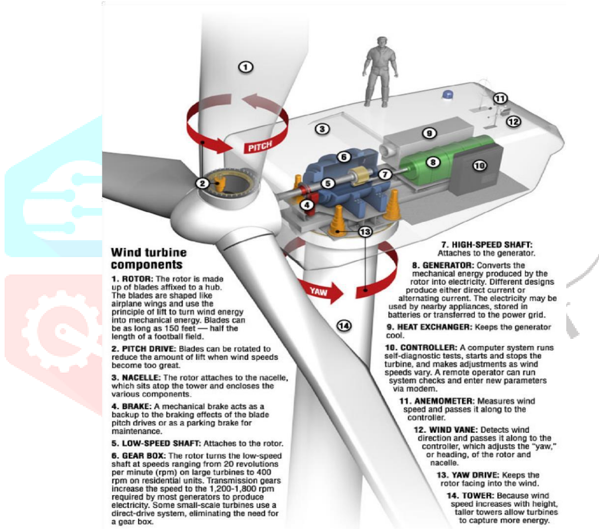
Figure 5. Typical configuration of a modern large scale wind turbine (www.desmoinesregister.com).
