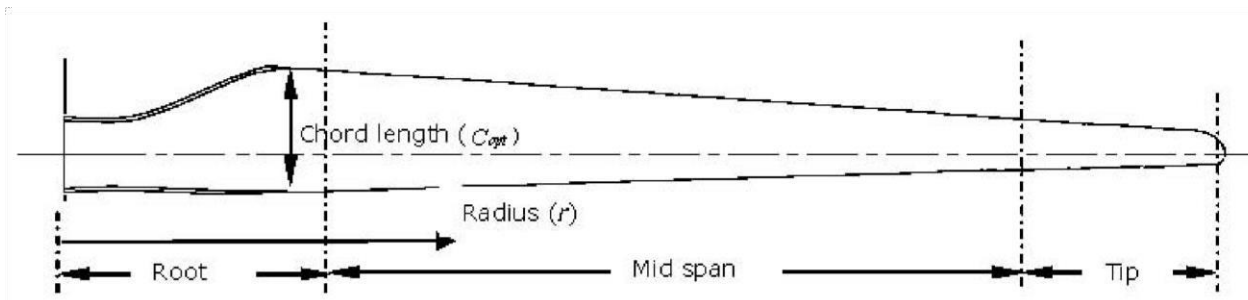
Figure 2. A typical blade plan and region classification.
