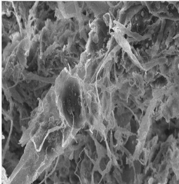
Figure.1 SEM monograph of virgin paper pulp sample “Balwaik Sumit A, Raut S P”, (2013)
