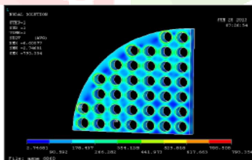
Figure 10 Von Misses Stress distributions across tube sheet of ASME heat exchanger
