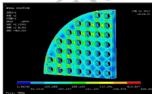
Figure 11 Von Misses Stress distribution across tube sheet of TEMA heat exchanger
