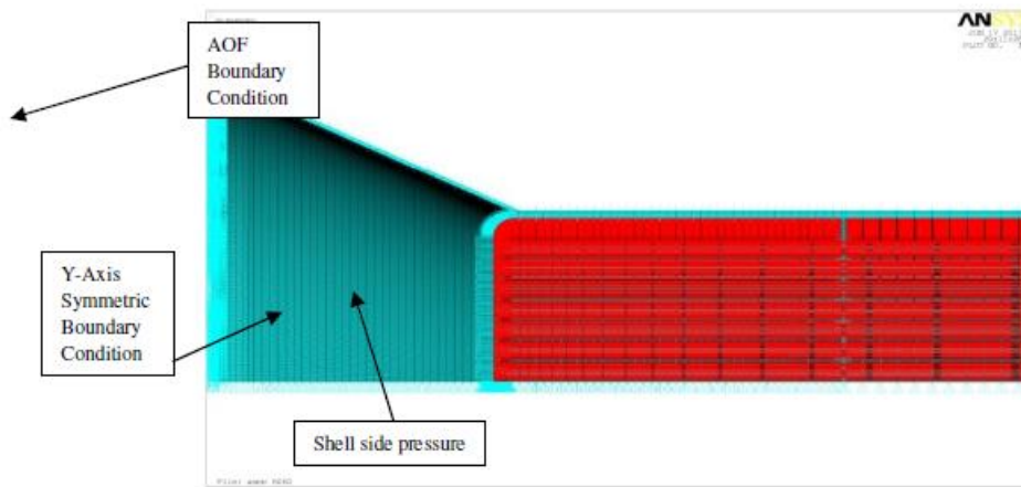
Fig.7 mechanical boundary condition applied on heat exchanger
