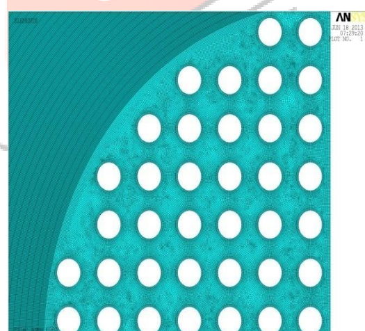
Figure 4 meshed model of TEMA heat exchanger
