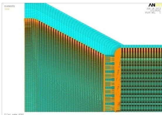
Fig.5 temperature applied at inner surface of heat exchanger
