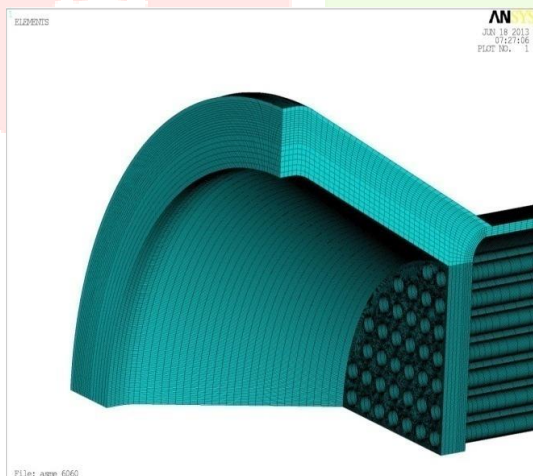
Figure 3 meshed model of ASME heat exchanger
