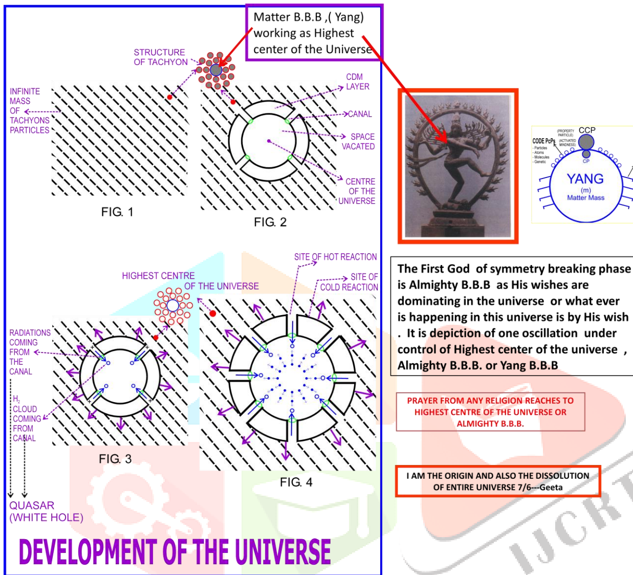
Figure 22 .1 Hoyle Narlikar Universe OR Universe "I"
