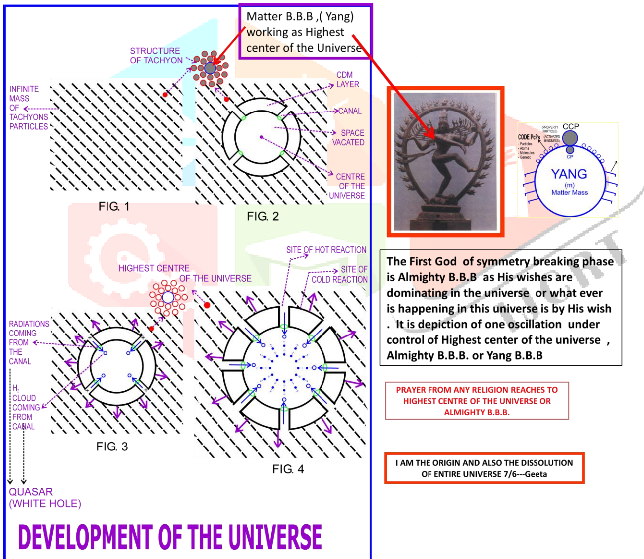
Figure 9.1 Hoyle Narlikar Universe OR Universe “I”
