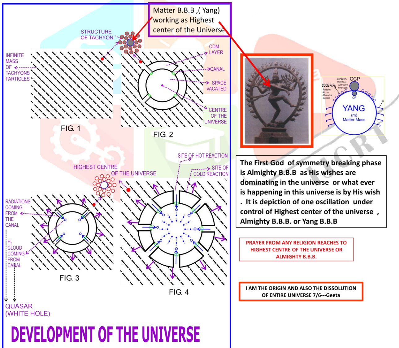
Figure 9.1 Hoyle Narlikar Universe OR Universe “T”
