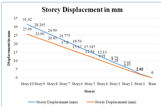
Fig 6: Displacement
