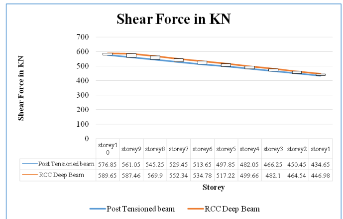
Fig4: Shear Force
