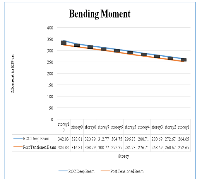
Fig 3: Bending Moment
