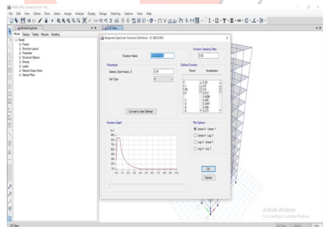
Figure 2 Seismic load
