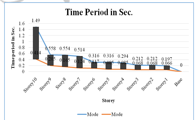
Fig 5: Time period
