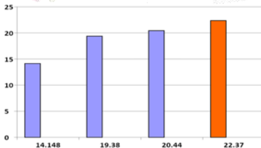
Figure: Compressive strength results of C-95:FA-5 with different volume fraction of CA&amp;RA
