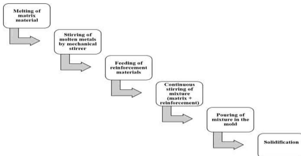
Fig.2.2 Flowchart of fabrication process
