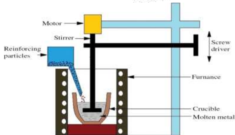
Fig.2.1 Stir casting process setup
