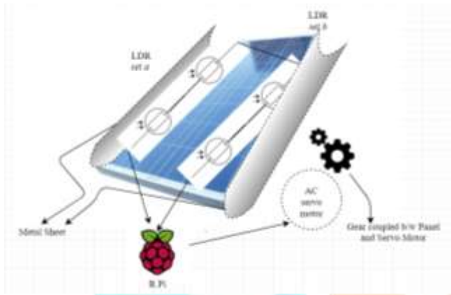
Fig 5 The experimental setup of the system
