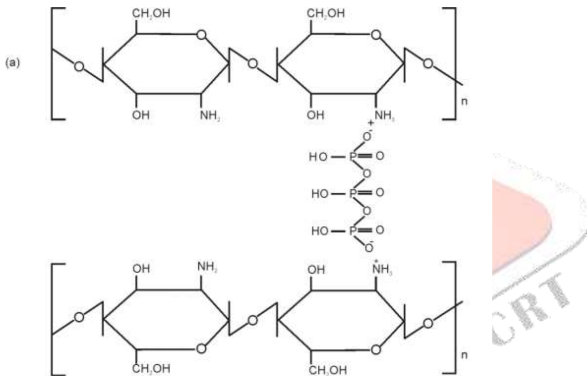
Fig. 1 (a) Chemical structure of cross - linking between chitosan and TPP in CTPP
