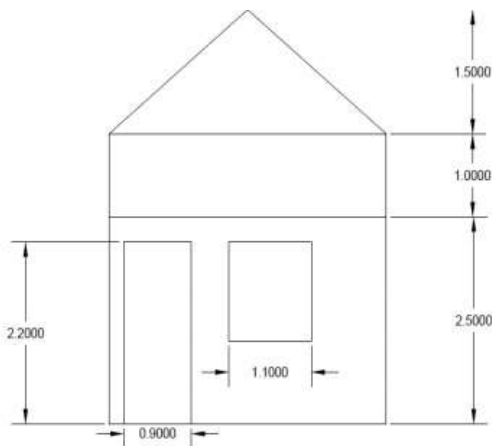
Fig. Front elevation plan
