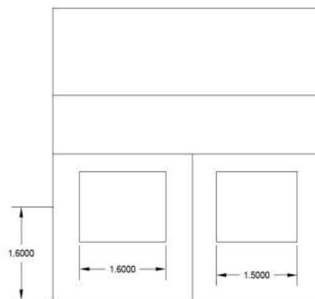
Fig. Right hand side view
