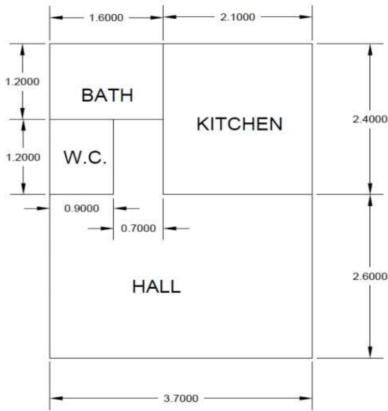
Fig. Floor plan
