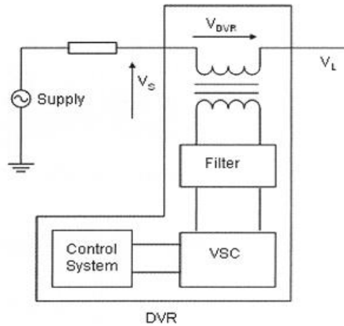
Fig.1.Schematic Diagram of DVR
