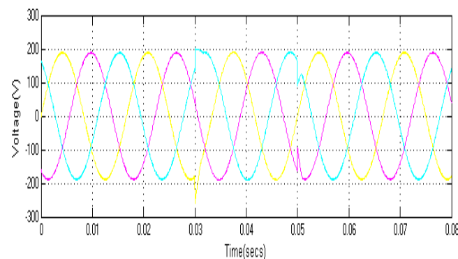
Fig.12 Load voltage.
