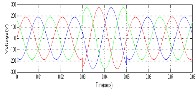
Fig .10Performance of DVR during Voltage swell
