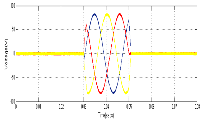
Fig.11 Voltage injected by the DVR during swell.
