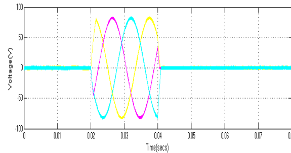
Fig.8 Voltage injected by the DVR during sag.
