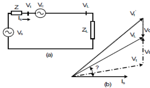
Fig.2 Equivalent Circuit diagram of DVR
