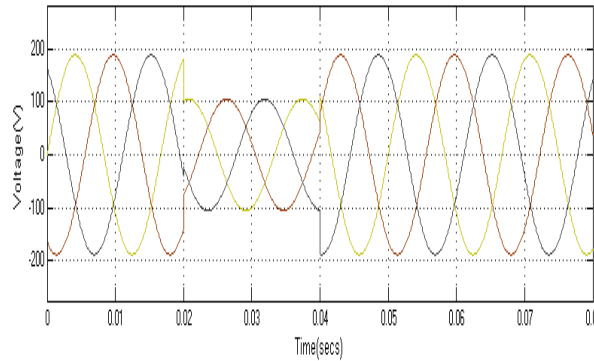
Fig.7 Performance of DVR during voltage sag.
