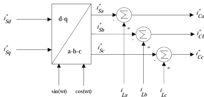
Fig.4 Generation of reference compensator currents
