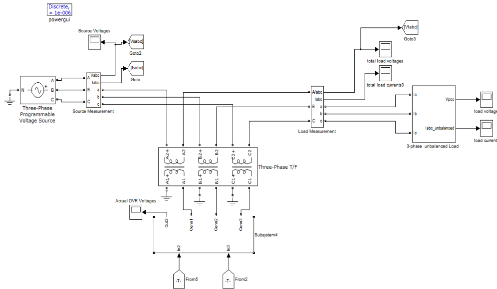
Fig. 5 MATLAB-based model of the Capacitor-supported DVR-connected system.
