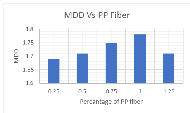
Figure: 8 bar chart Variation of MDD with % of PPF
