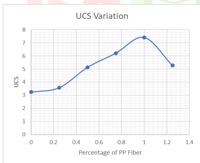
Figure: 9 Variation of unconfined compressive strength with % of PPF
