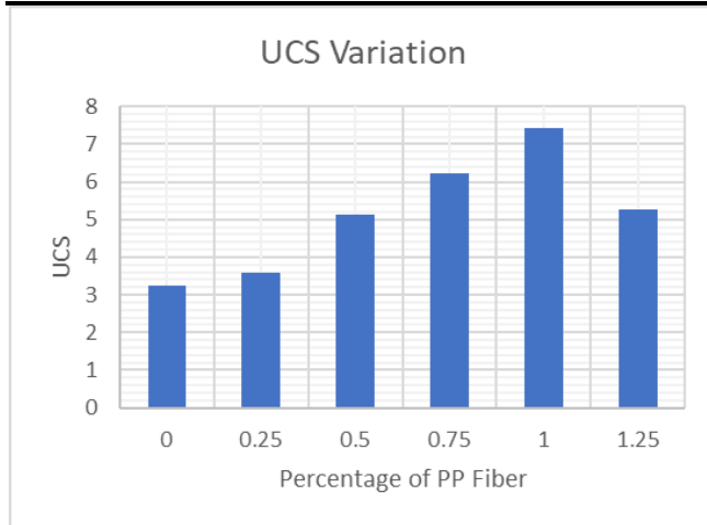
Fig:-10 Bar chart Variation of UCS with % of PPF
