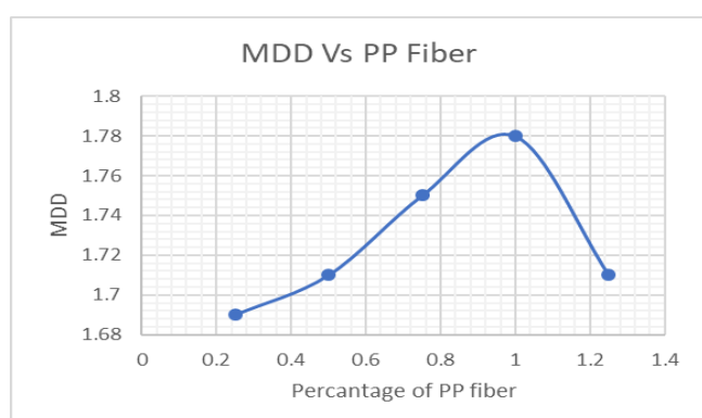
Figure:-7 Variation of MDD with % of PPF
