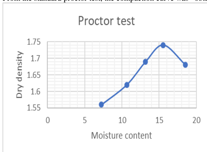
Figure: 1 moisture content-dry density curve
