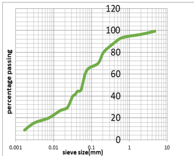
Figure: 2 Grain size distribution curve of natural soil
