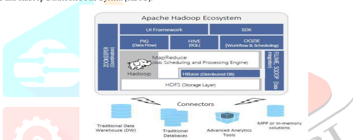
Figure 6: HDFS Architecture
