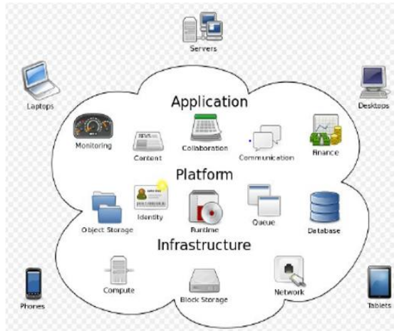
Figure 3: Cloud Computing
