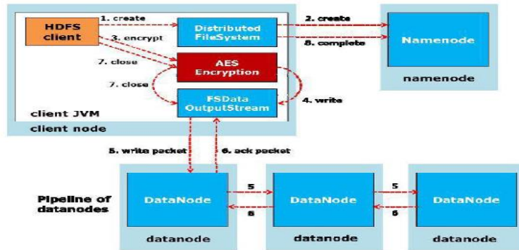
Figure 11: Encryption Process
