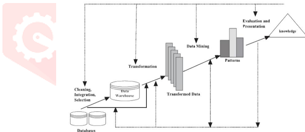
Figure 4: Knowledge-Discovery Process
