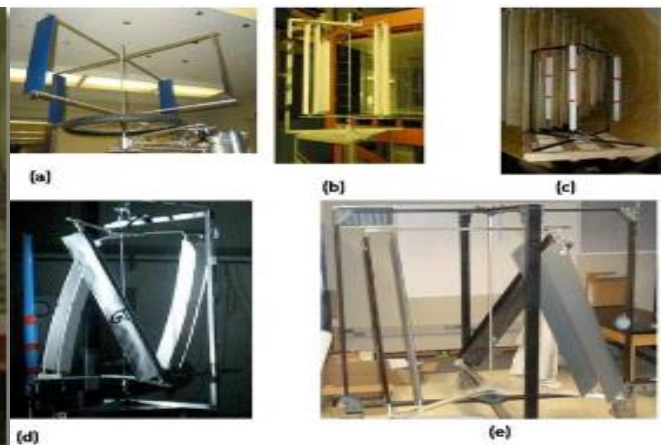
Figure.9. Different models of Vertical Axis Wind Turbine
