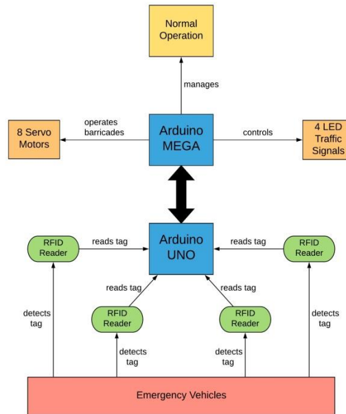
Figure 6: Architectural block diagram
