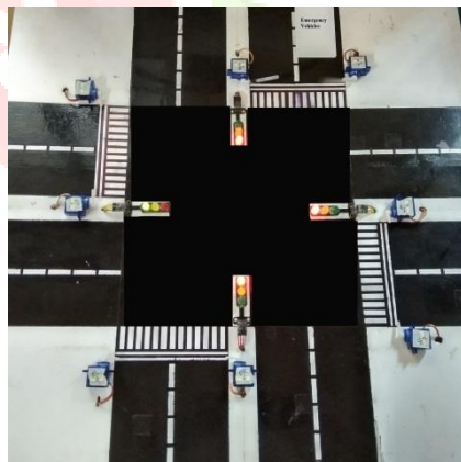
Figure 7(a): Road Junction Model
