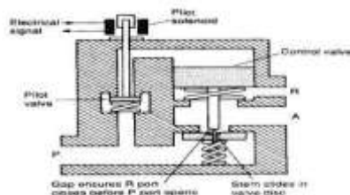
Figure 4.17 Construction of a pilot-operated 3/2 valve
