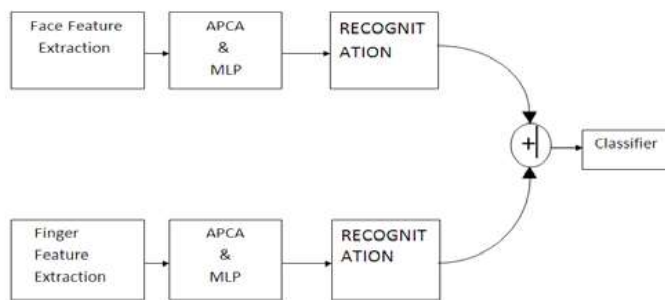
Figure 2.1 : Neural network classifier
