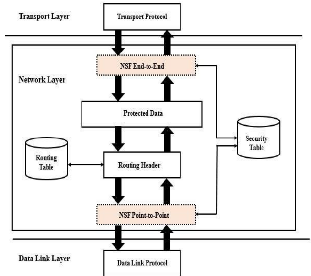
Figure 1: Diagram illustrating the NSF confidentiality, integrity and authentication services for data packets.
