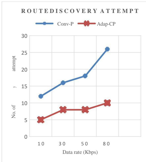
Figure 3. Route discover attempt of Conv-P and Adap-CP forstatic network.
