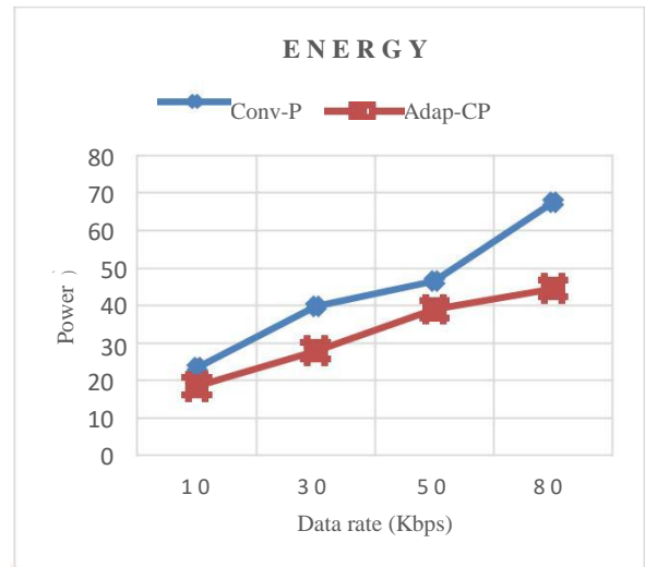
Figure 4. Energy consumption of Conv-P and Adap-CP forstatic network.
