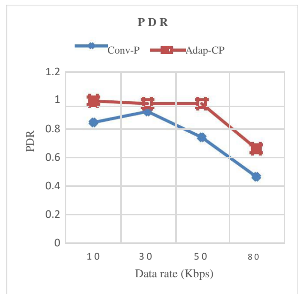
Figure 2. PDR of Conv-P and Adap-CP for static network.
