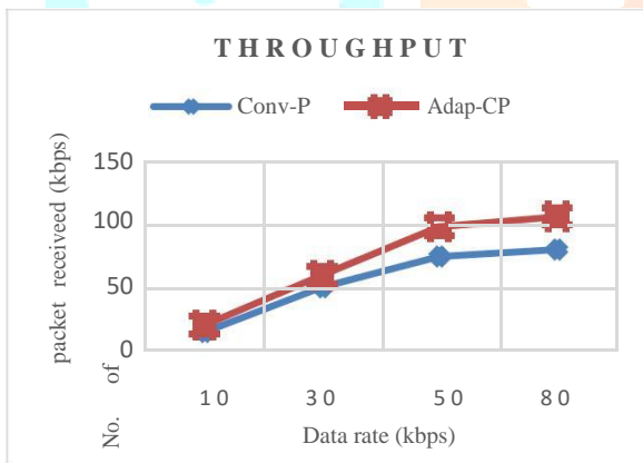
Figure 1. Throughput of Conv-P and Adap-CP for static network.
